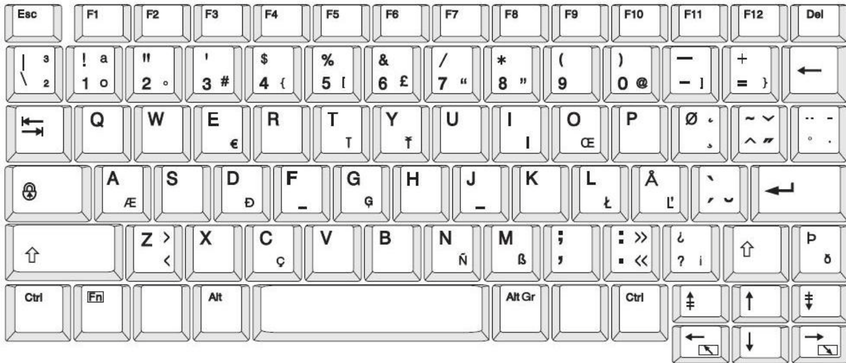
Figure 4. QWERTY – EU-Tastaturkonfiguration
